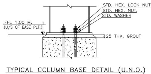
TYPICAL COLUMN BASE DETAIL (U.N.O.)
