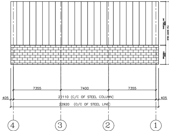
SIDEWALL SHEETING ELEVATION ALONG GRID LINE 1
