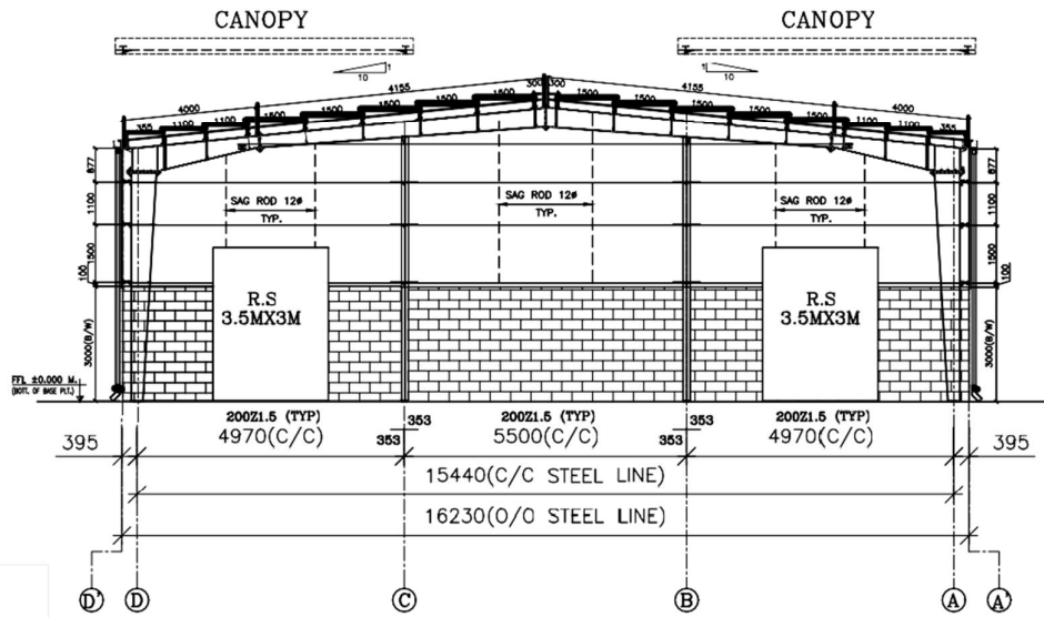
FRAMING ELEVATION (FOR GRID LINE 7 ) ALL PURLIN/GIRTS 200 Z 1.5 (TYP)
