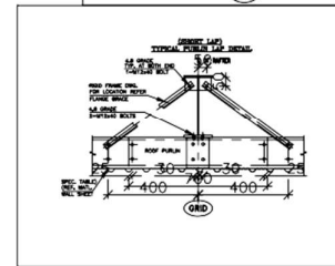
SECTION B
