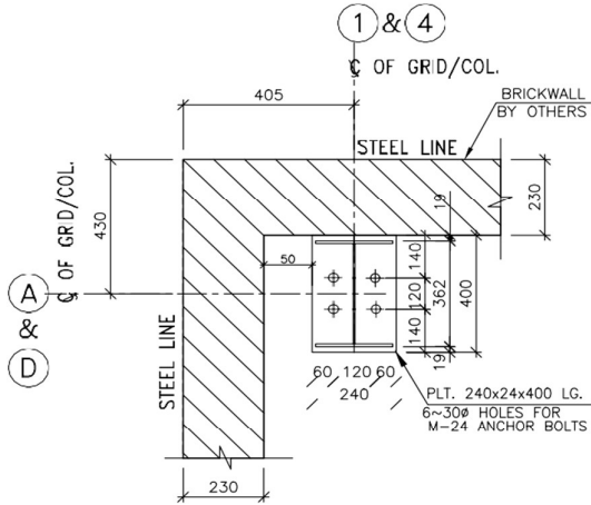
DETAIL D1 (02 No. REQD.) GA-01 (AS DRAWN)
