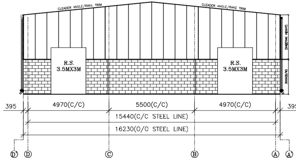
98 END WALL SHEETING ELEVATION (FOR GRID LINE 7)
