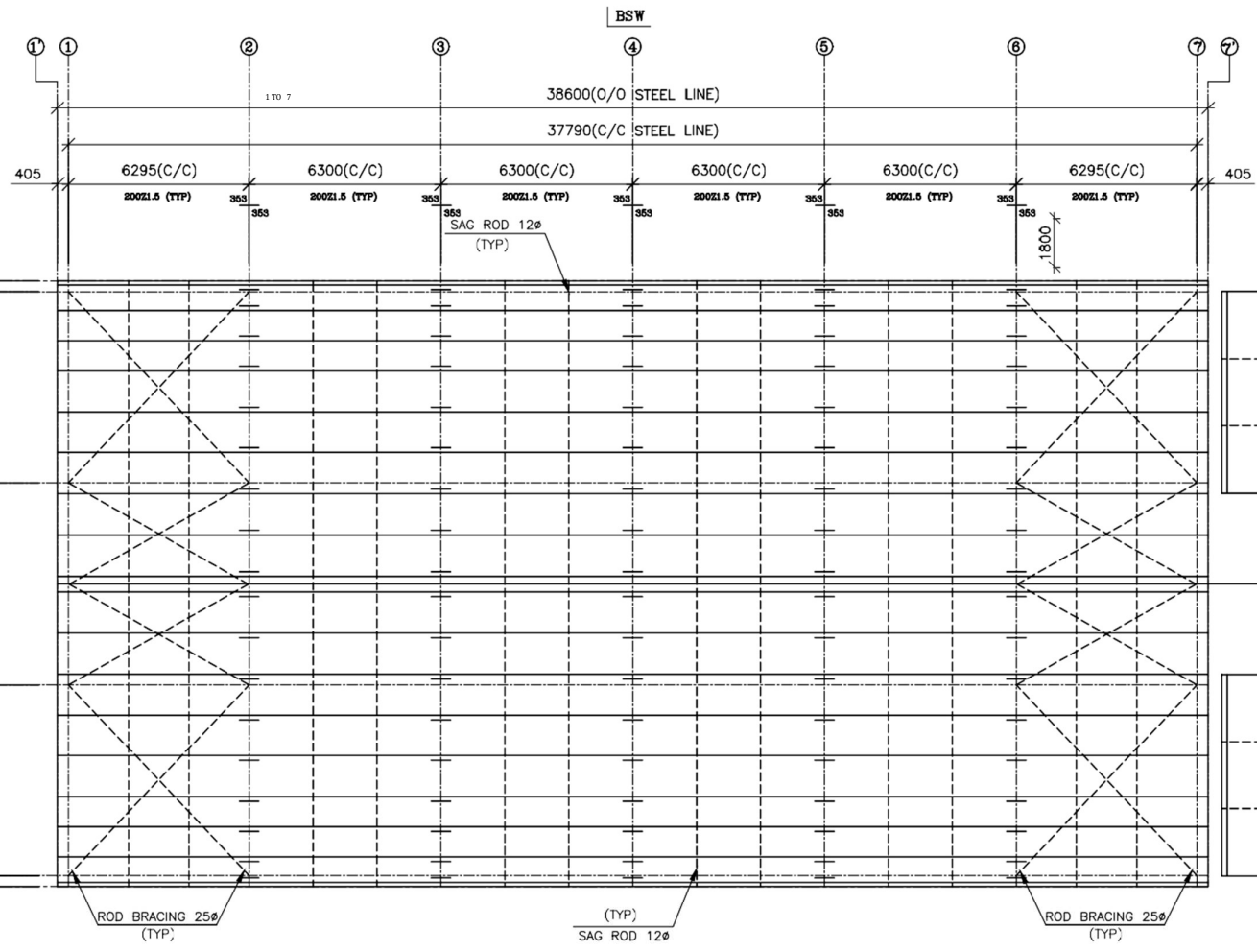
ROOF FRAMING PLAN ALL PURLIN/GIRT 200Z1.5 TYP
