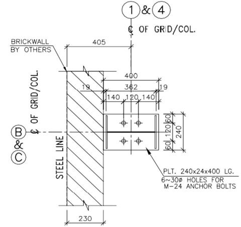
DETAIL D3 (02 Nos. REQD.) GA-01 (AS DRAWN)
