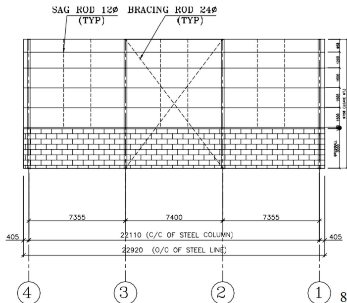
SIDEWALL FRAMING ELEVATION ALONG GRID LINE A
