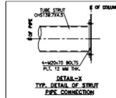
DETAIL OF STRUT PIPE CONNECTION
