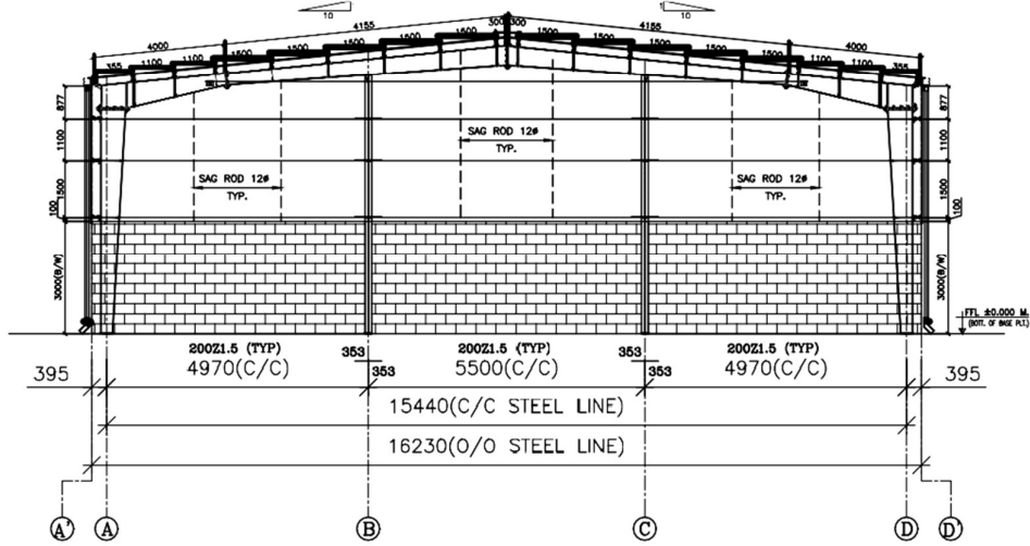
FRAMING ELEVATION (FOR GRID LINE 1 ) ALL PURLIN/GIRTS 200 Z 1.5 (TYP)
