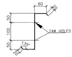
TYPICAL PURLIN DETAIL
