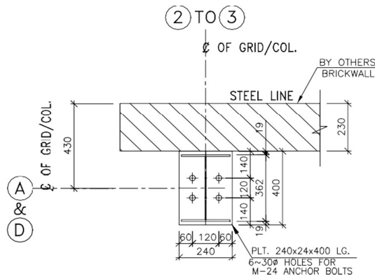
DETAIL D2 (02 Nos. REQD.) GA-01 (AS DRAWN)
