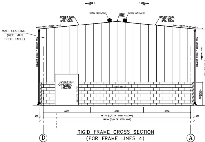
RIGID FRAME CROSS SECTION (FOR FRAME LINES 1)
